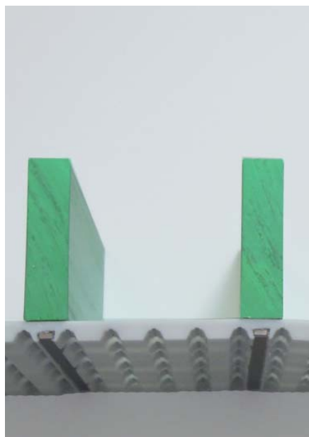
Mechanically mounted profiles
